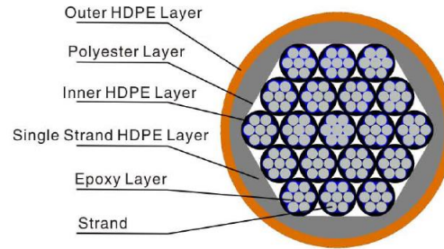
Epoxy Filled Tendon Cable
