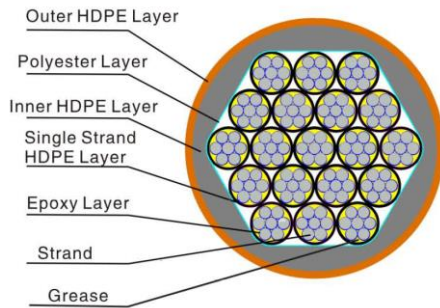
Galvanized+Single Epoxy Coated Tendon Cable
